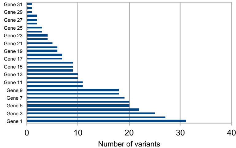
GWAS variants distribution
